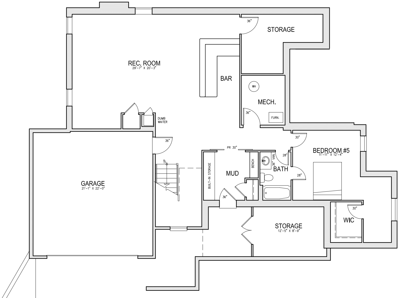
FINISHED BASEMENT PLAN
